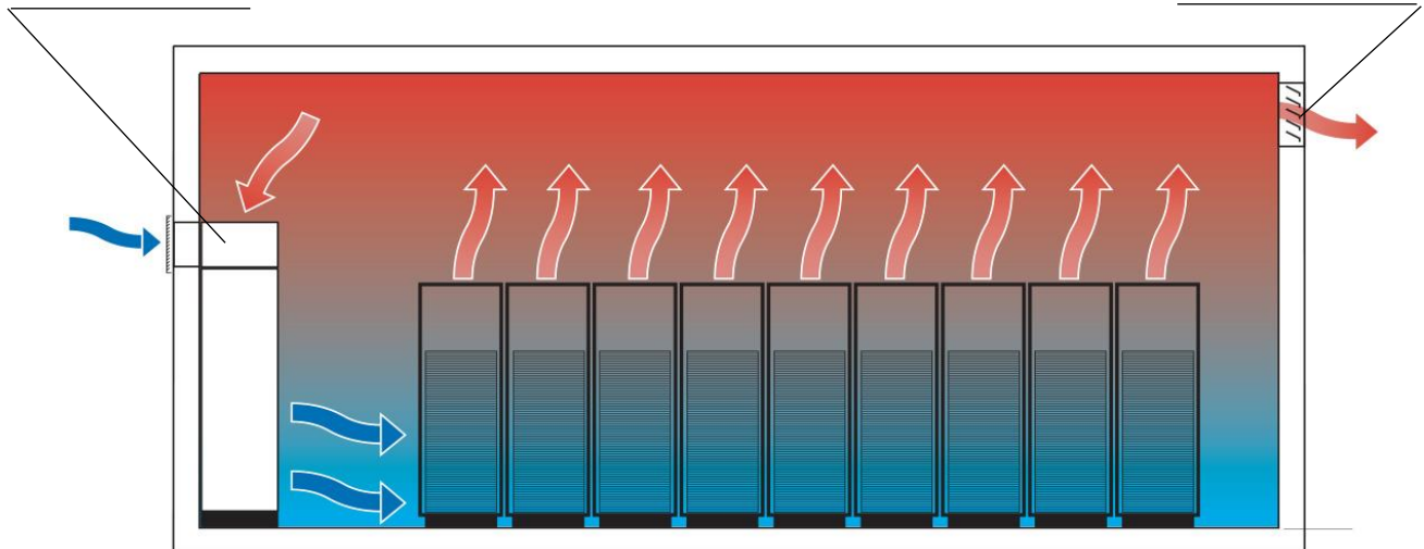
FREE-COOLING plenum
